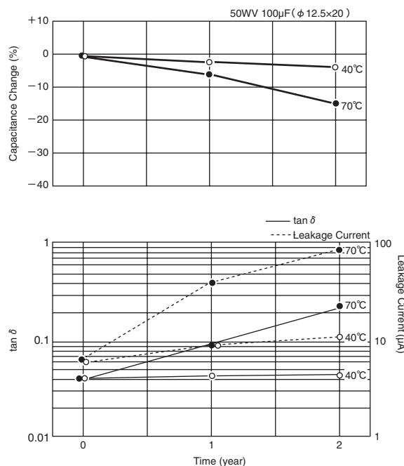
Fig-30 Temperature Characteristics of Storage
