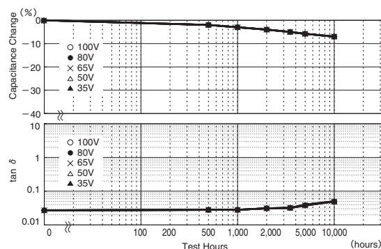
Fig-20 Endurance (measured by each apply voltage, result curves are overlapped)
